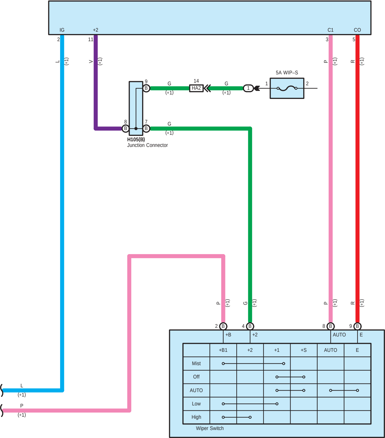
H25(B) Windshield Wiper Switch Assembly
